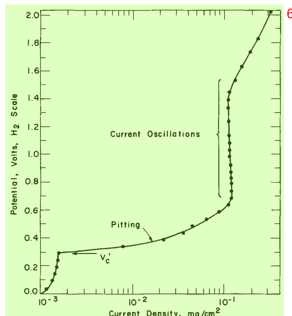
Fig. 4. Potentiostatic anodic polarization curve for 15% Cr, 13% Ni stainless steel in 0.1N NaCl, 25^\circ\text{C} .
