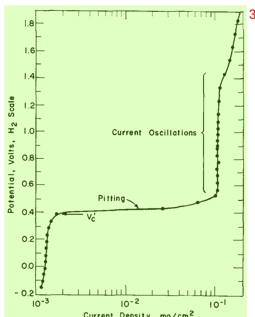
Fig. 7. Potentiostatic anodic polarization curve for 15% Cr, 13% Ni, 1.43% Mo stainless steel in 0.1N NaCl, 25°C.
