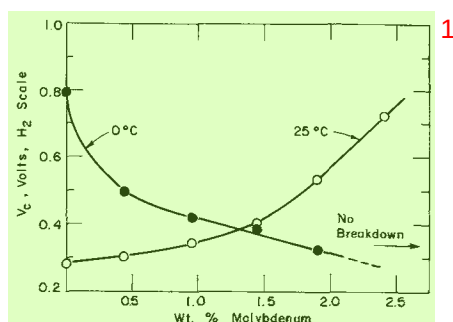
Fig. 6. Critical pitting potentials for 15% Cr, 13% Ni stainless steel with increasing Mo content, in 0.1N NaCl, 25°C and 0°C.
