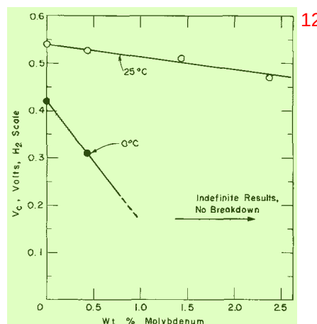
Fig. 8. Critical pitting potentials for 15% Cr, 13% Ni stainless steel with increasing Mo content in 0.1N NaBr, 25°C and 0°C.
