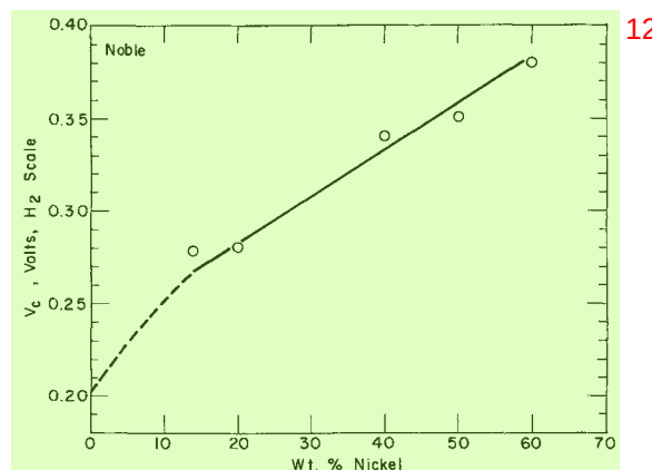
Fig. 5. Critical pitting potentials for 15% Cr-Fe alloys with increasing Ni content, in 0.1\text{N NaCl} , 25^\circ\text{C} .
